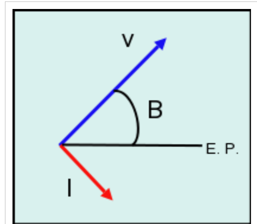
Figura 4. Diagrama fasorial.
